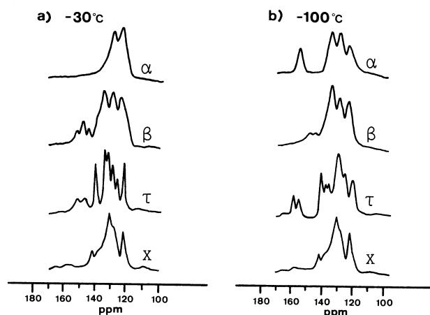
Fig. 2. Solid-state ^{13}\text{C} NMR spectra of four kinds of metal-free phthalocyanines using the CP-MAS method. a) -30^\circ\text{C} , b) -100^\circ\text{C} .
